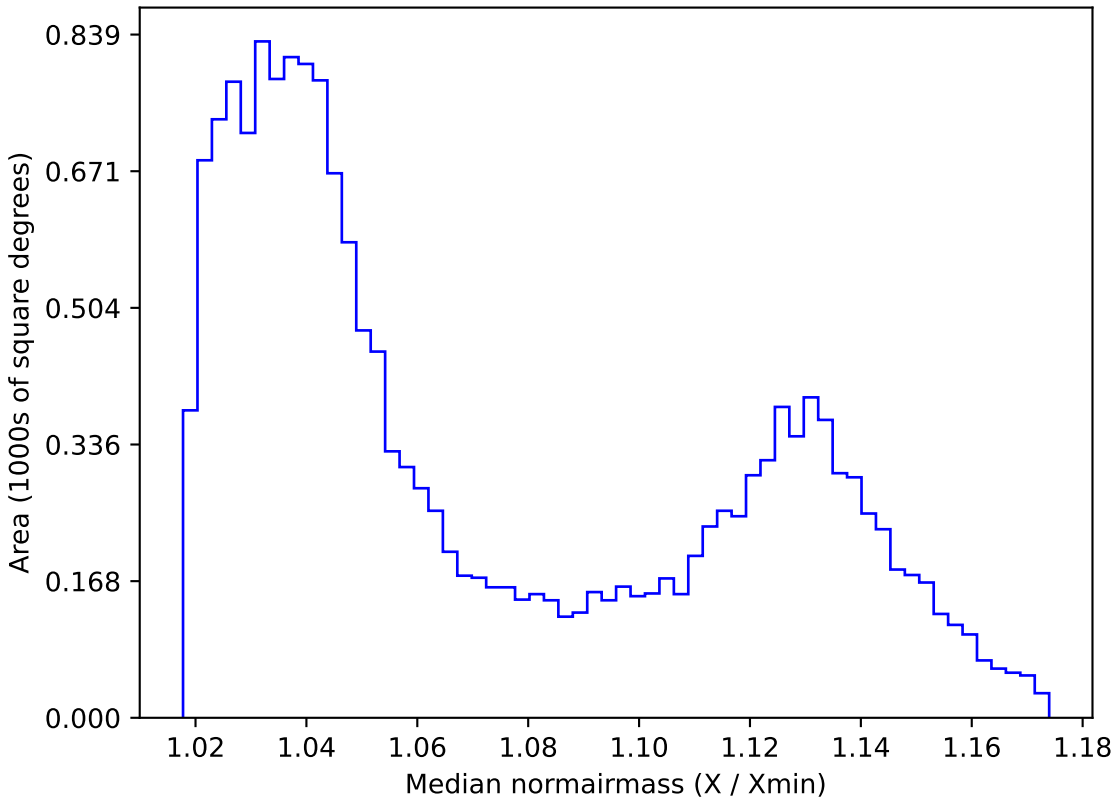
roll_pause_mjdp270_v3.4_10yrs WFD r band: Median normairmass
