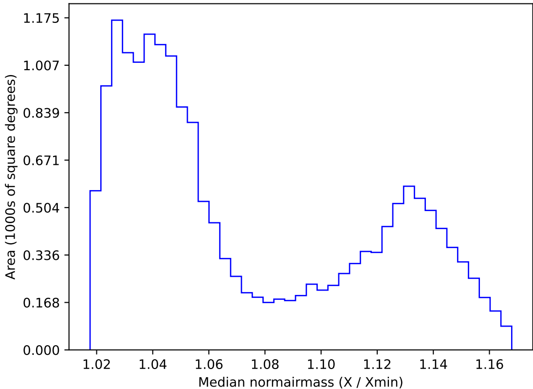
roll_pause_mjdp270_v3.4_10yrs WFD i band: Median normairmass
