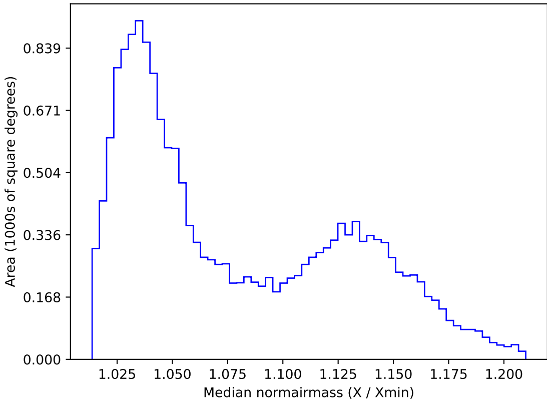
roll_pause_mjdp270_v3.4_10yrs WFD g band: Median normairmass
