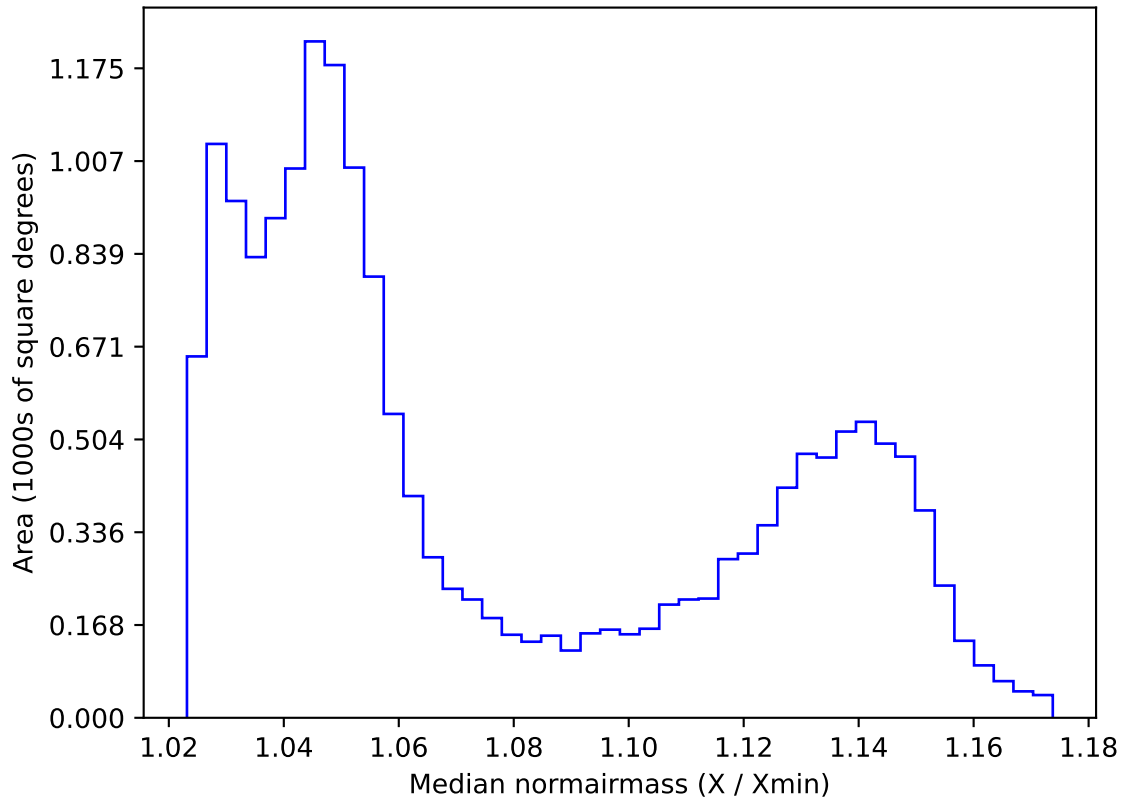
roll_pause_mjdp270_v3.4_10yrs WFD all bands: Median normairmass
