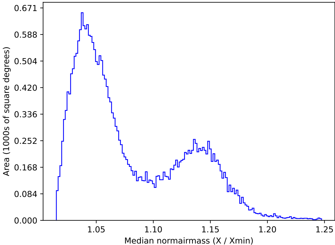
roll_pause_mjdp270_v3.4_10yrs All sky z band: Median normairmass
