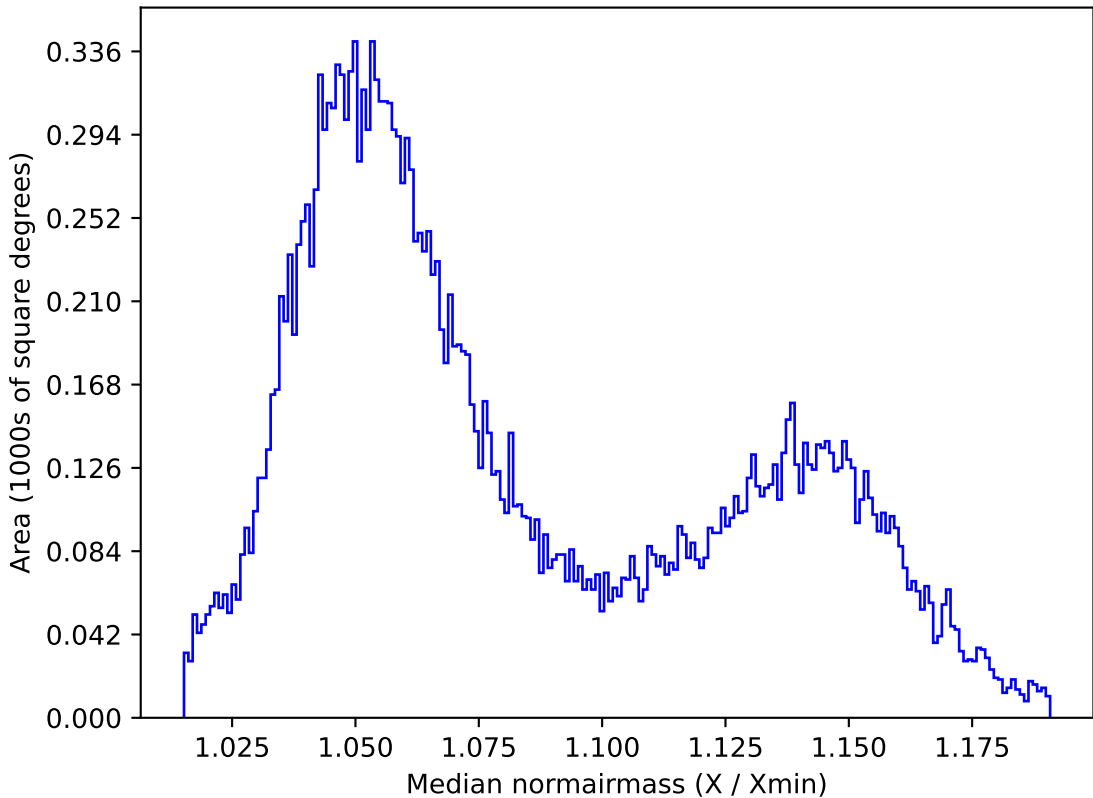
roll_pause_mjdp270_v3.4_10yrs All sky y band: Median normairmass
