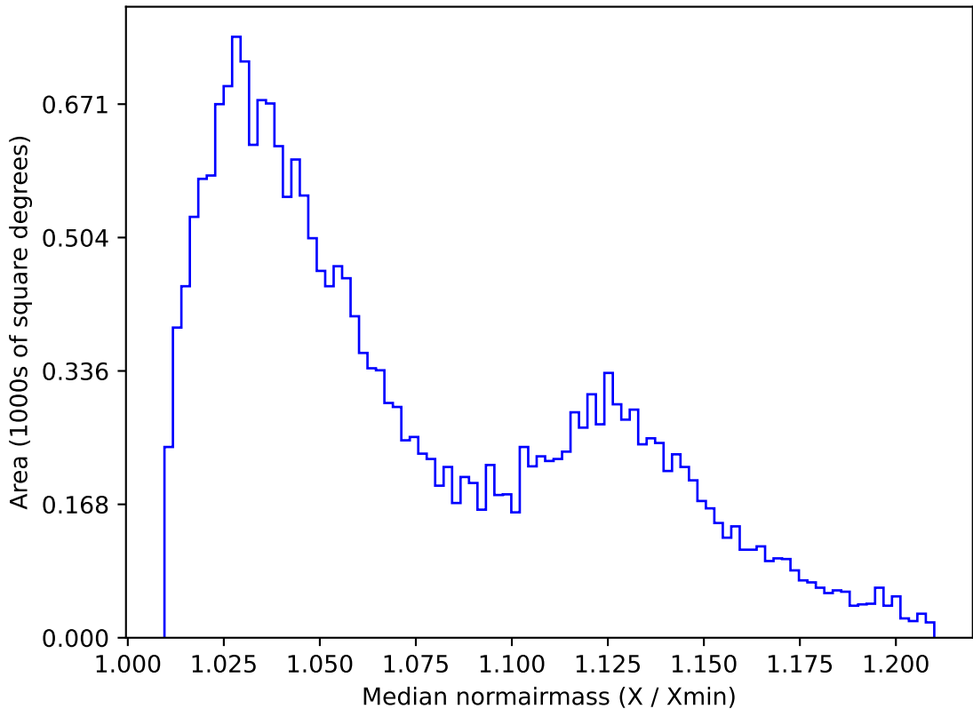
roll_pause_mjdp270_v3.4_10yrs All sky u band: Median normairmass
