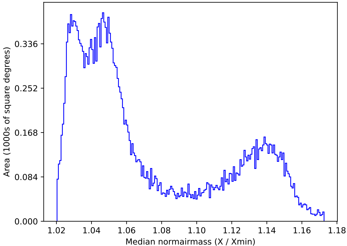
roll_pause_mjdp270_v3.4_10yrs All sky all bands: Median normairmass
