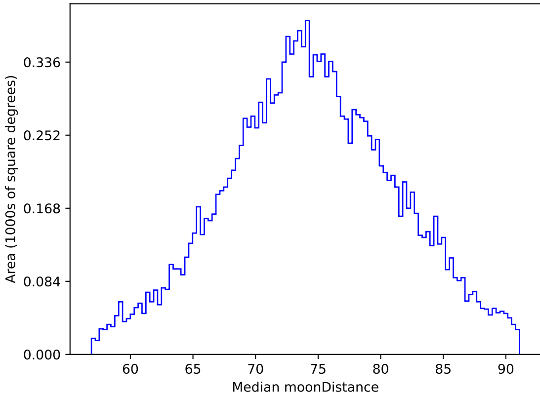
roll_pause_mjdp270_v3.4_10yrs WFD z band: Median moonDistance
