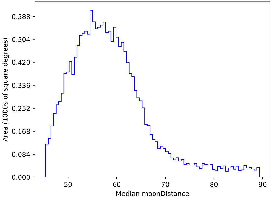
roll_pause_mjdp270_v3.4_10yrs WFD y band: Median moonDistance
