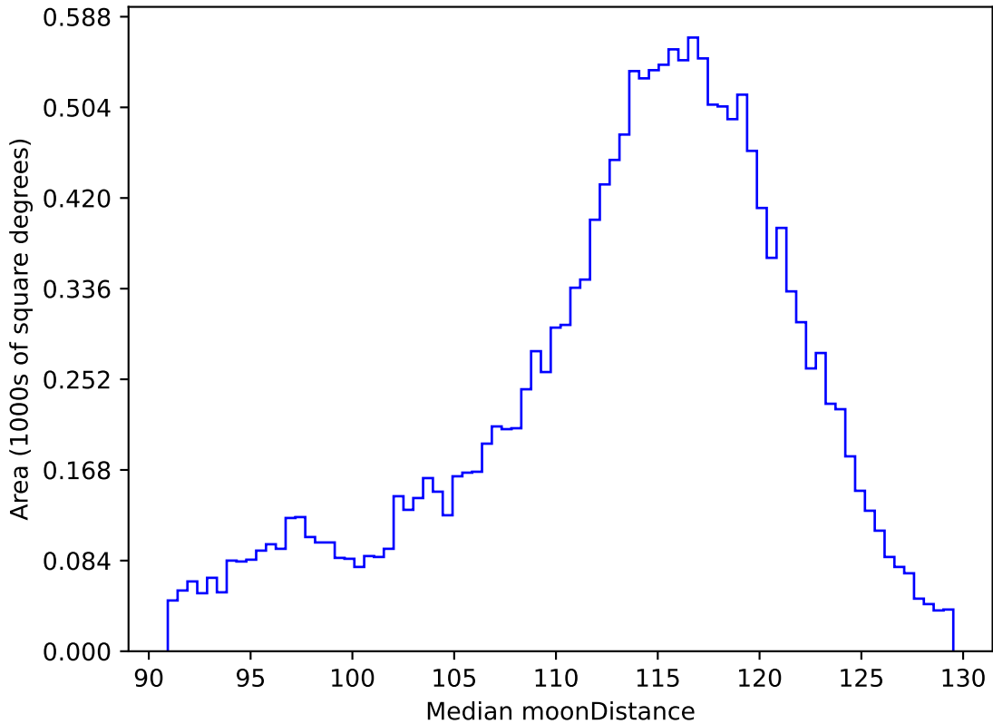
roll_pause_mjdp270_v3.4_10yrs WFD r band: Median moonDistance
