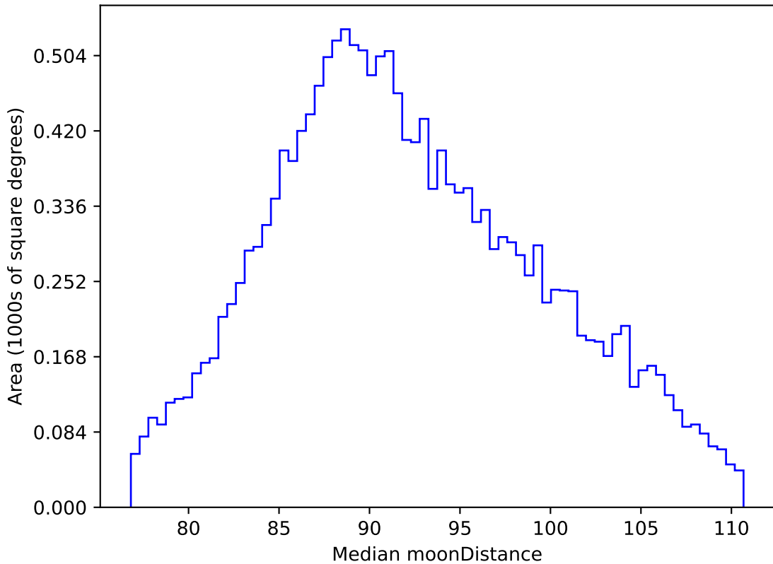
roll_pause_mjdp270_v3.4_10yrs WFD i band: Median moonDistance
