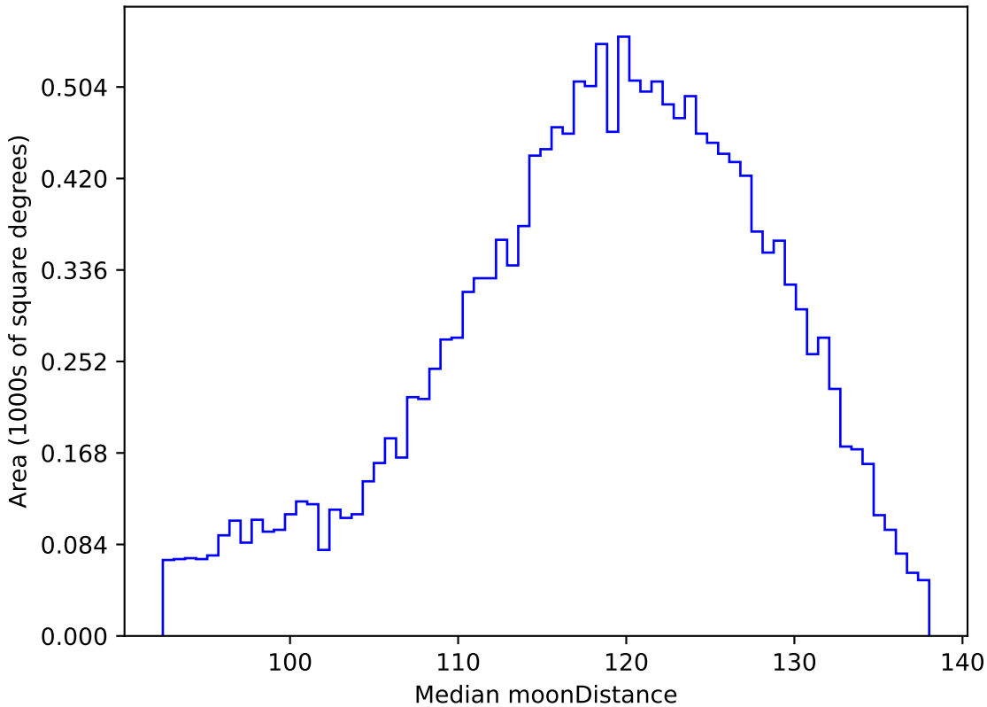
roll_pause_mjdp270_v3.4_10yrs WFD g band: Median moonDistance
