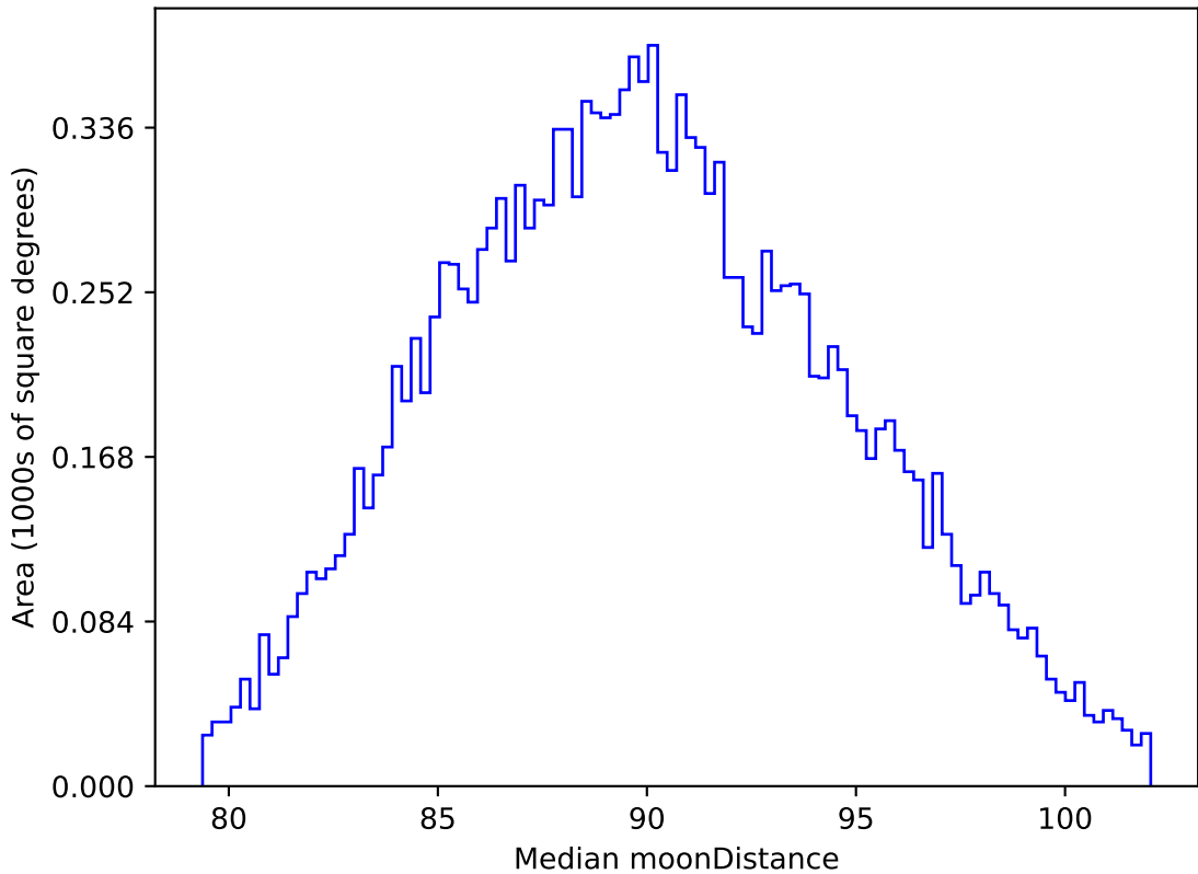
roll_pause_mjdp270_v3.4_10yrs WFD all bands: Median moonDistance
