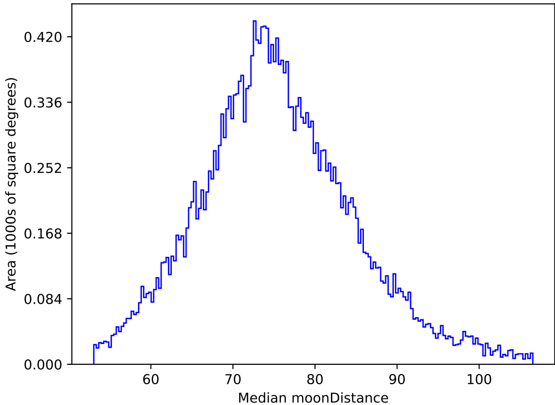
roll_pause_mjdp270_v3.4_10yrs All sky z band: Median moonDistance
