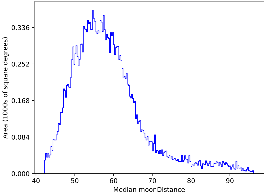
roll_pause_mjdp270_v3.4_10yrs All sky y band: Median moonDistance
