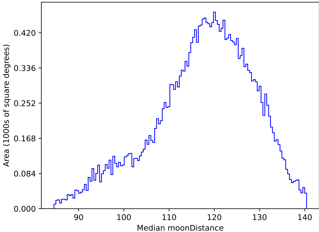
roll_pause_mjdp270_v3.4_10yrs All sky g band: Median moonDistance
