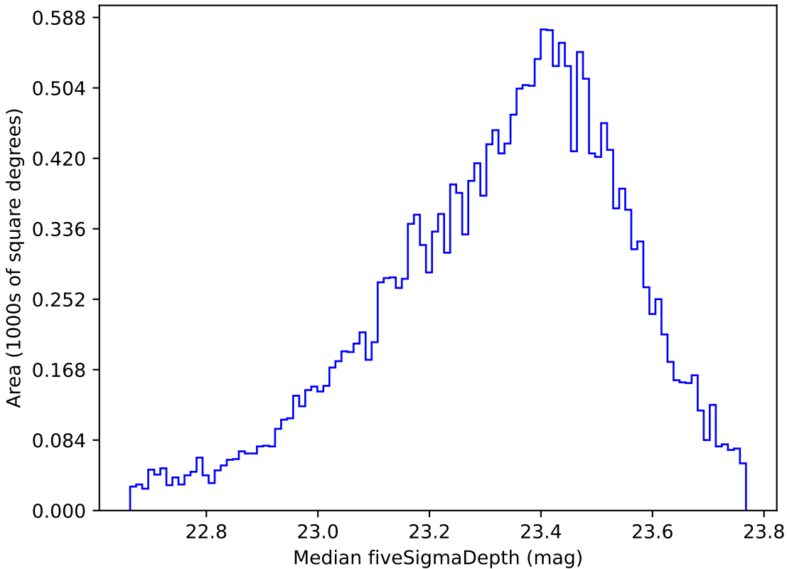
roll_pause_mjdp270_v3.4_10yrs Yr 1 u band: Median fiveSigmaDepth
