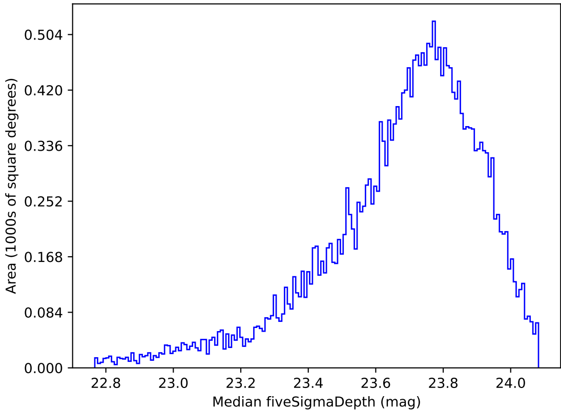
roll_pause_mjdp270_v3.4_10yrs Yr 1 i band: Median fiveSigmaDepth
