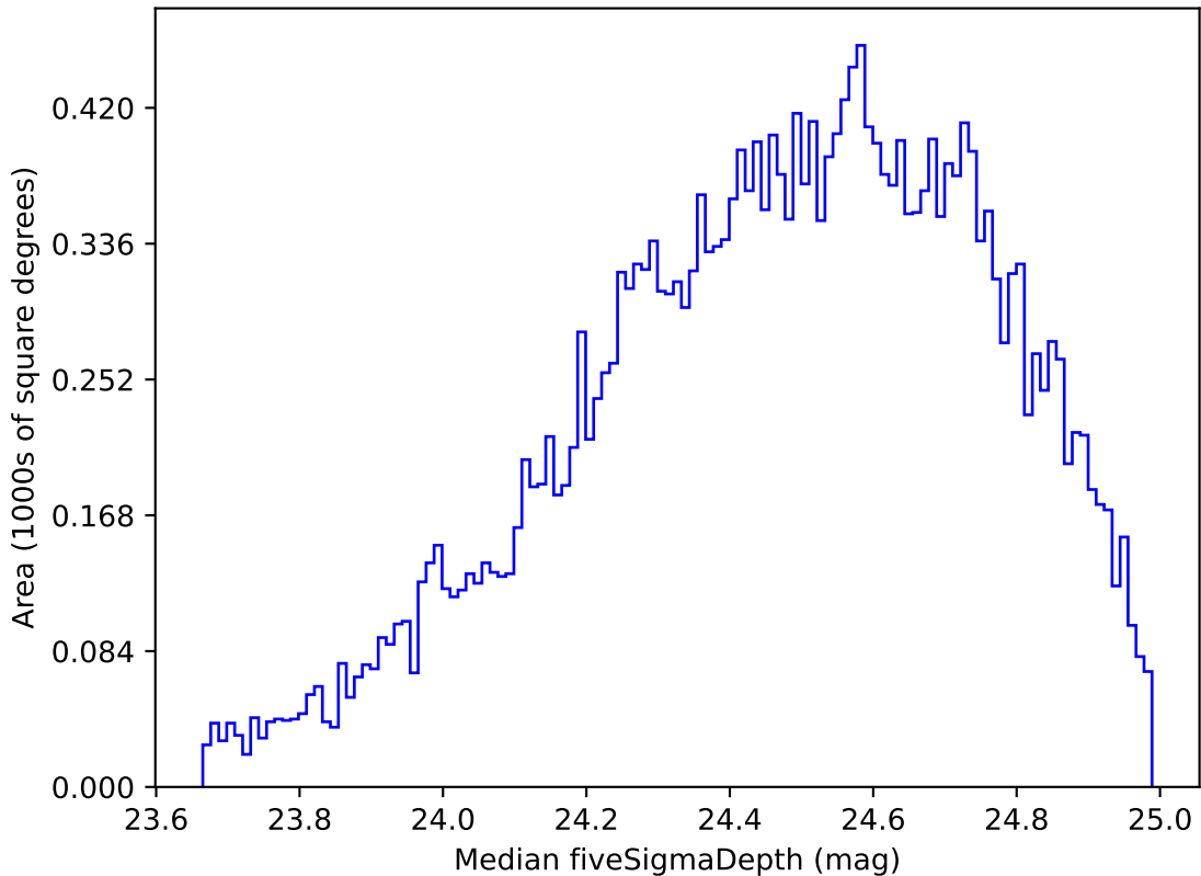
roll_pause_mjdp270_v3.4_10yrs Yr 1 g band: Median fiveSigmaDepth
