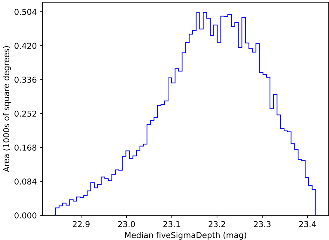
roll_pause_mjdp270_v3.4_10yrs WFD u band: Median fiveSigmaDepth
