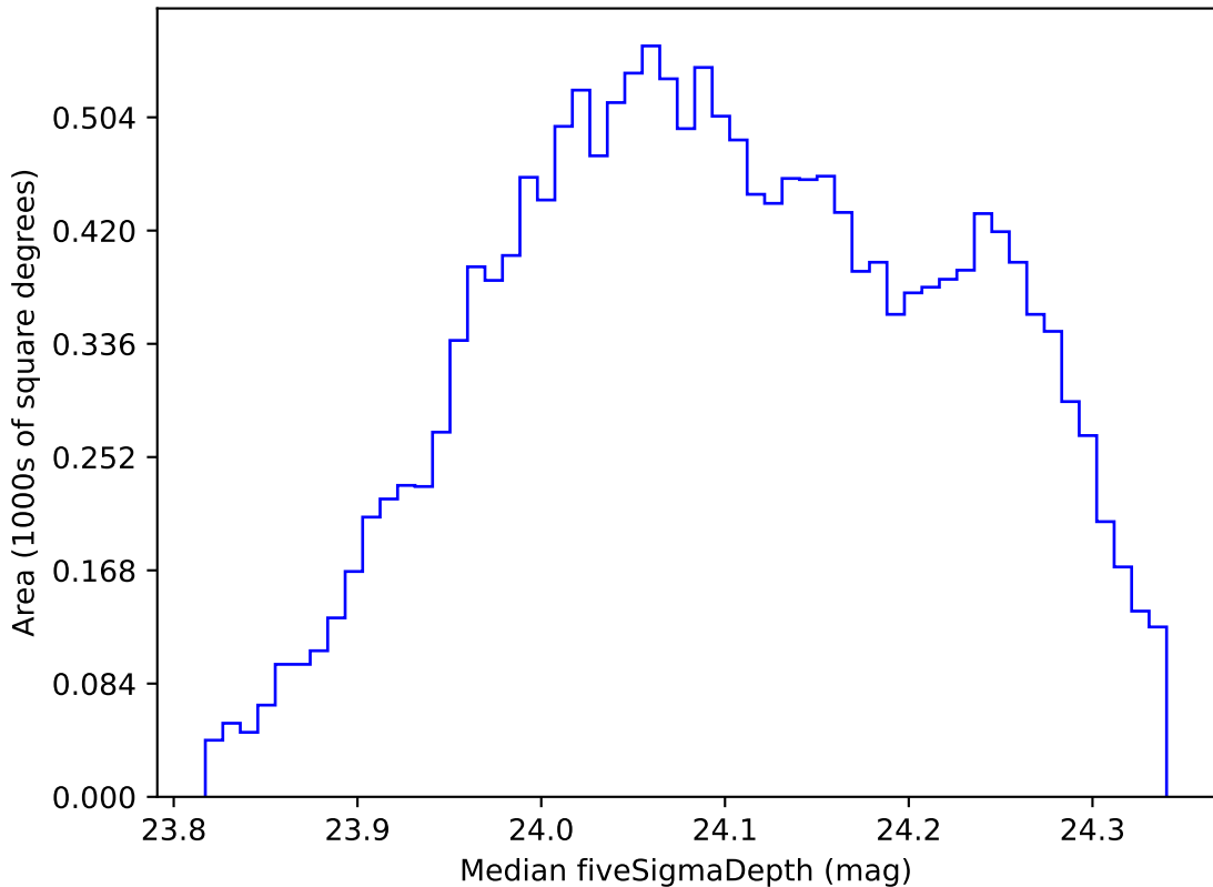
roll_pause_mjdp270_v3.4_10yrs WFD r band: Median fiveSigmaDepth
