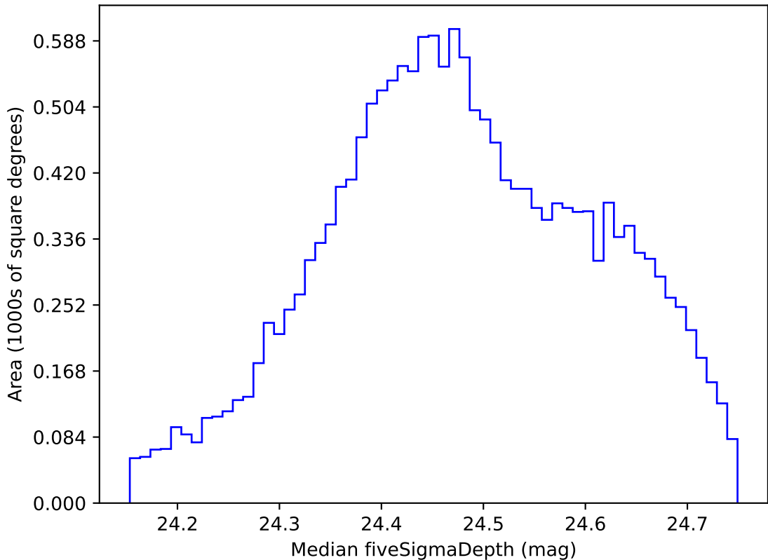
roll_pause_mjdp270_v3.4_10yrs WFD g band: Median fiveSigmaDepth
