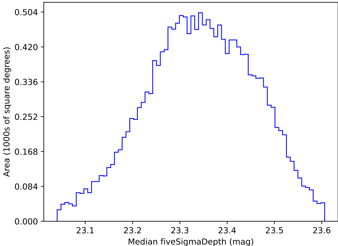
roll_pause_mjdp270_v3.4_10yrs WFD all bands: Median fiveSigmaDepth
