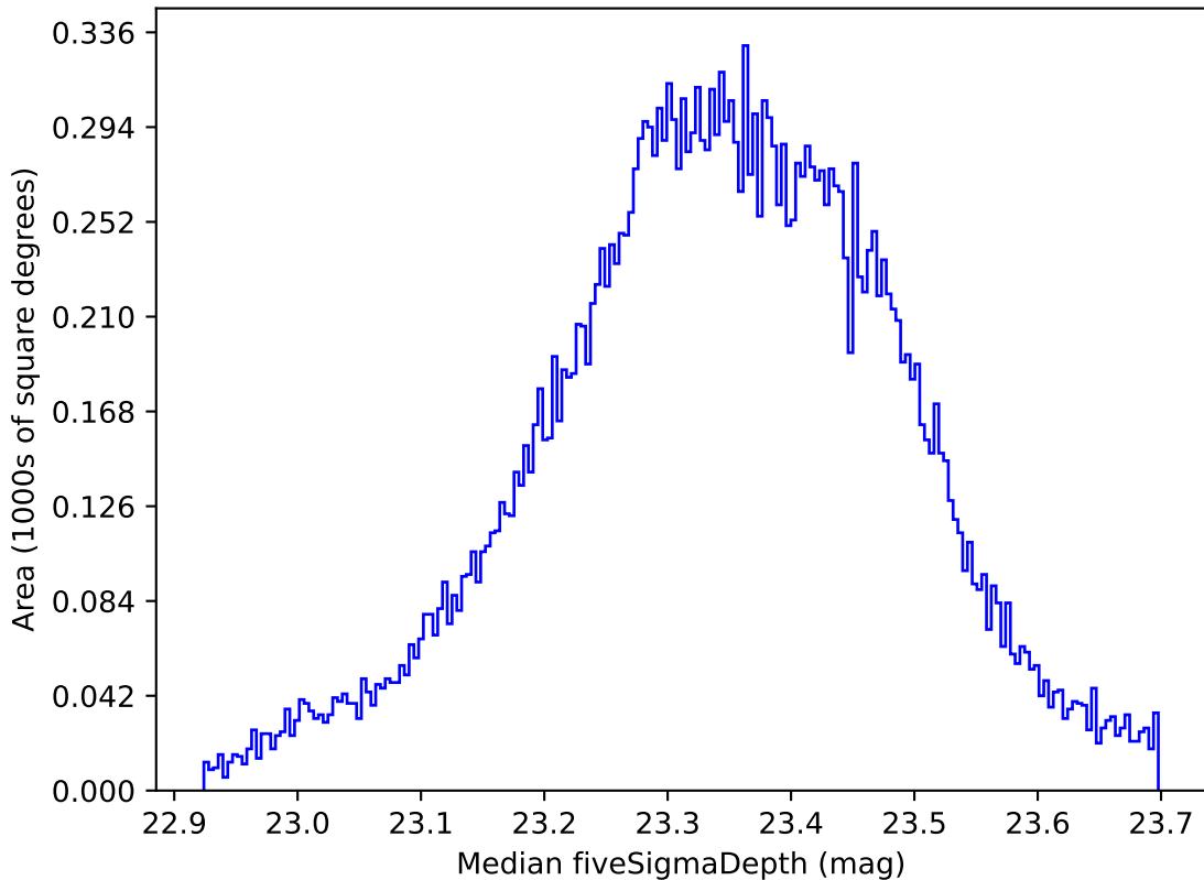
roll_pause_mjdp270_v3.4_10yrs All sky all bands: Median fiveSigmaDepth
