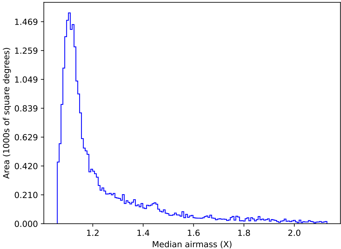
roll_pause_mjdp270_v3.4_10yrs Yr 1 i band: Median airmass
