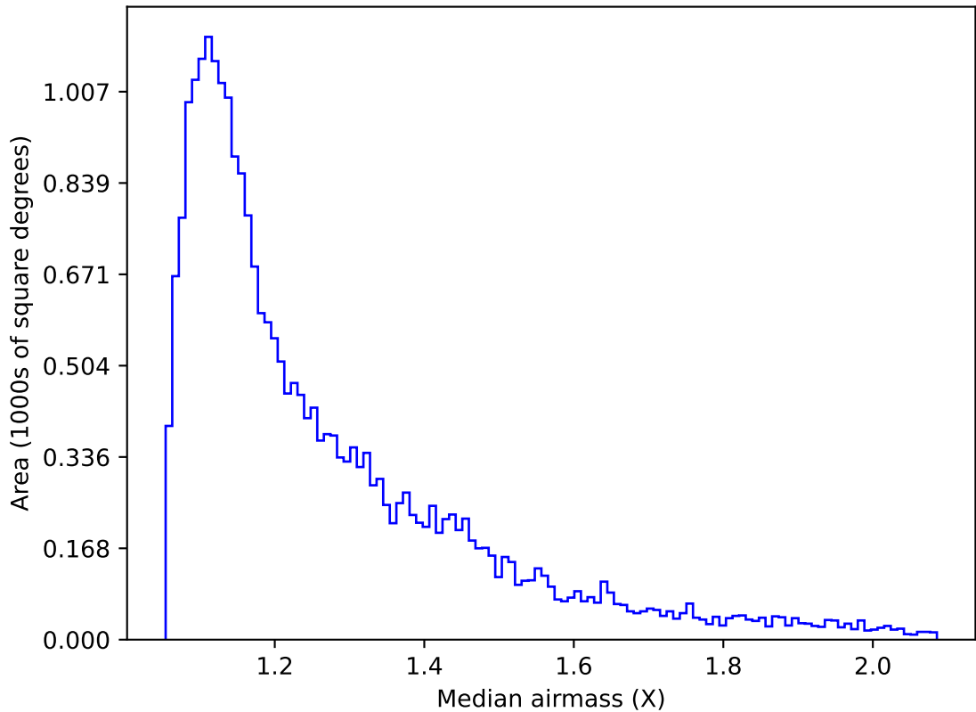
roll_pause_mjdp270_v3.4_10yrs Yr 1 g band: Median airmass
