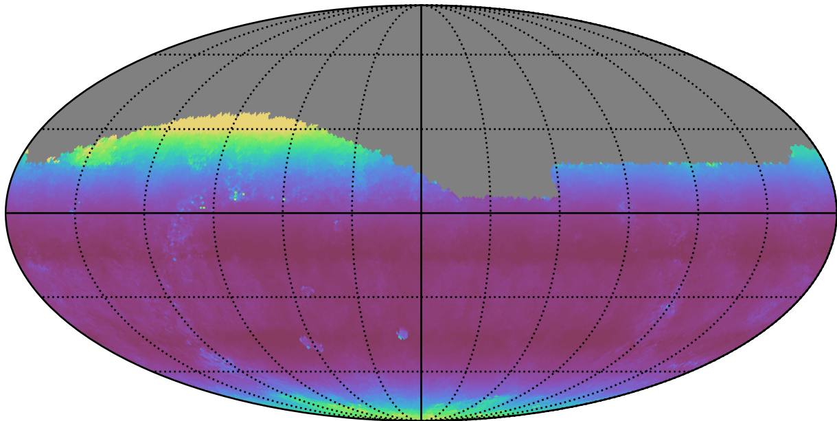
roll_pause_mjdp270_v3.4_10yrs Yr 1 all bands: Median airmass
