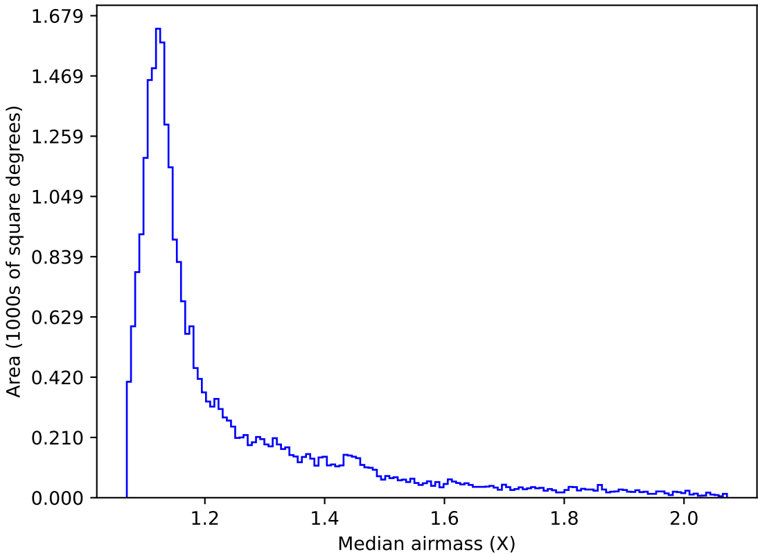
roll_pause_mjdp270_v3.4_10yrs Yr 1 all bands: Median airmass
