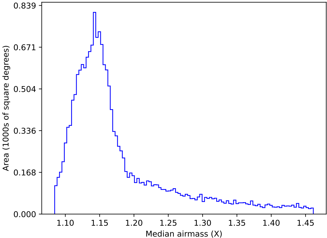
roll_pause_mjdp270_v3.4_10yrs WFD z band: Median airmass
