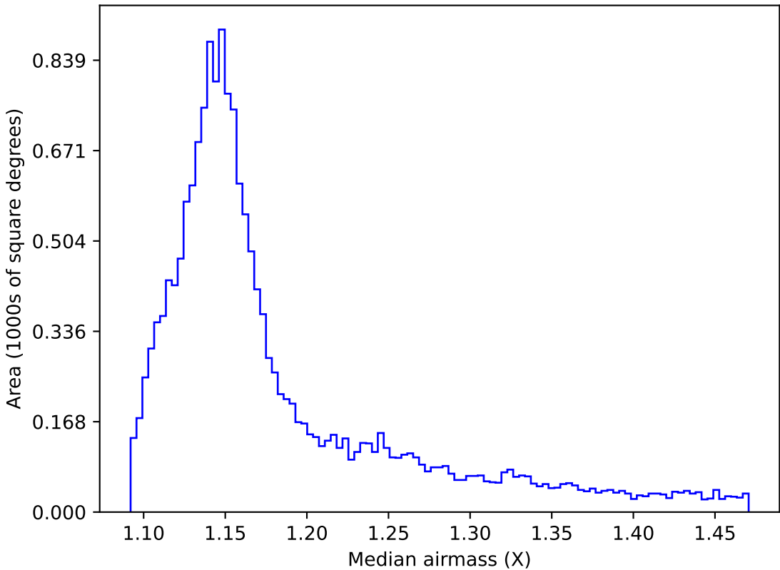
roll_pause_mjdp270_v3.4_10yrs WFD y band: Median airmass
