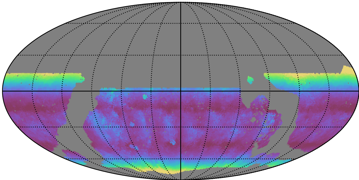
roll_pause_mjdp270_v3.4_10yrs WFD u band: Median airmass
