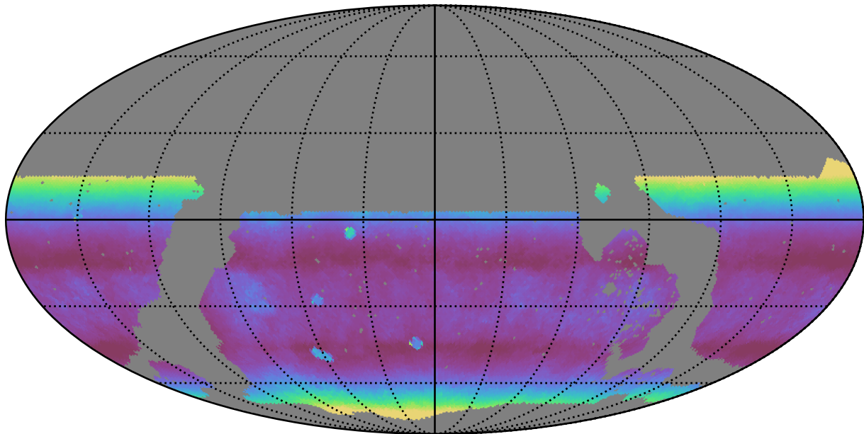
roll_pause_mjdp270_v3.4_10yrs WFD r band: Median airmass
