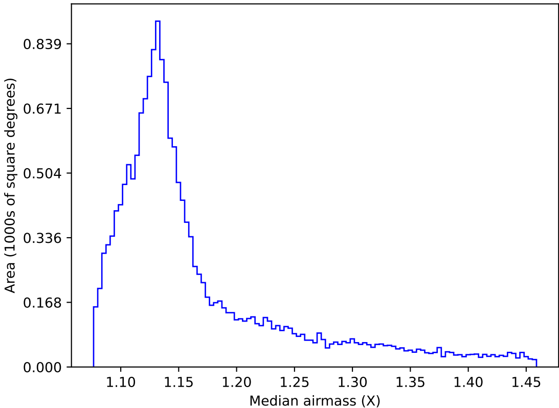
roll_pause_mjdp270_v3.4_10yrs WFD r band: Median airmass
