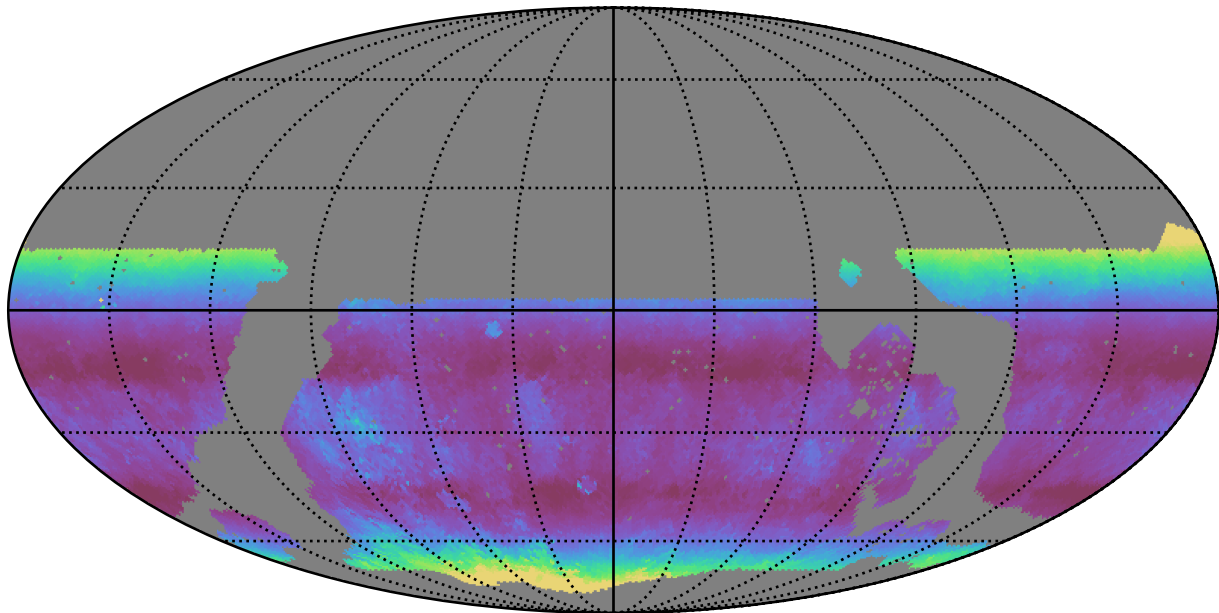
roll_pause_mjdp270_v3.4_10yrs WFD g band: Median airmass
