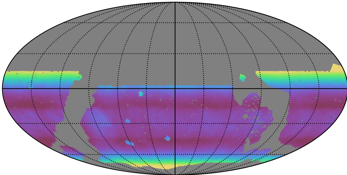
roll_pause_mjdp270_v3.4_10yrs WFD all bands: Median airmass
