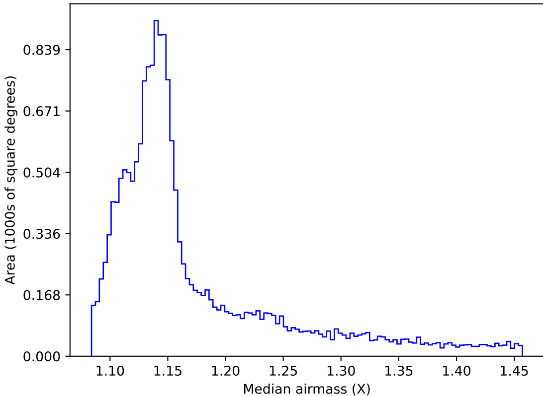
roll_pause_mjdp270_v3.4_10yrs WFD all bands: Median airmass
