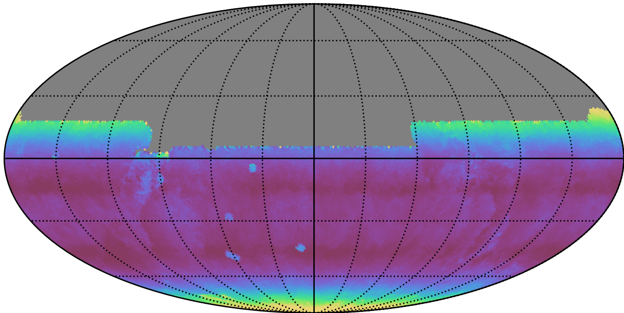
roll_pause_mjdp270_v3.4_10yrs All sky y band: Median airmass
