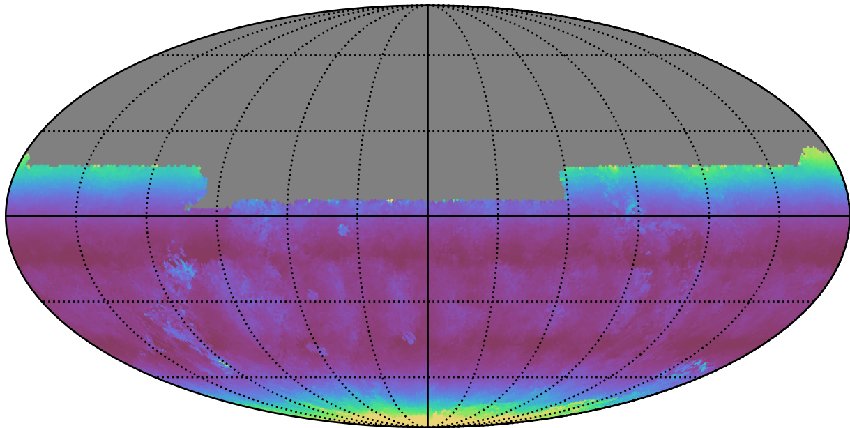
roll_pause_mjdp270_v3.4_10yrs All sky u band: Median airmass
