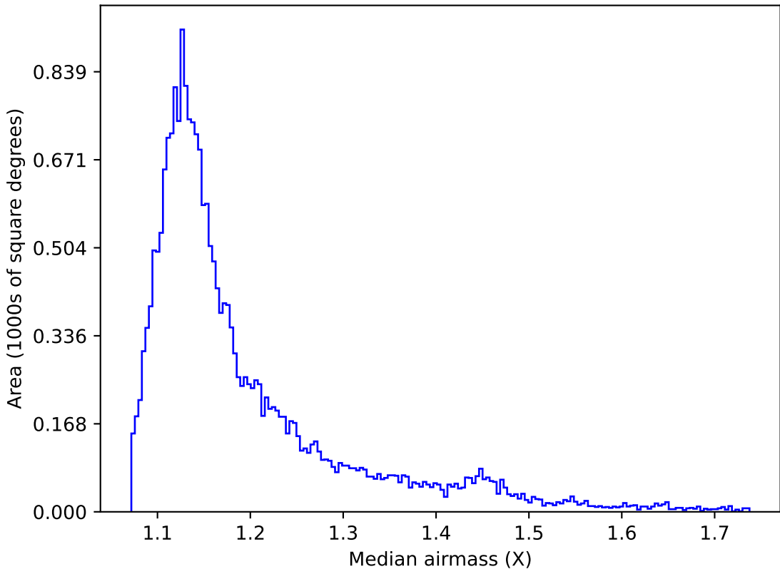
roll_pause_mjdp270_v3.4_10yrs All sky u band: Median airmass
