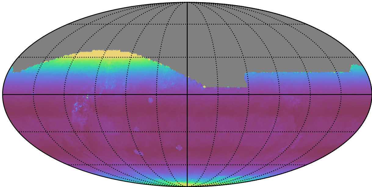
roll_pause_mjdp270_v3.4_10yrs All sky r band: Median airmass
