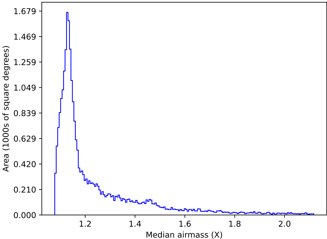
roll_pause_mjdp270_v3.4_10yrs All sky r band: Median airmass
