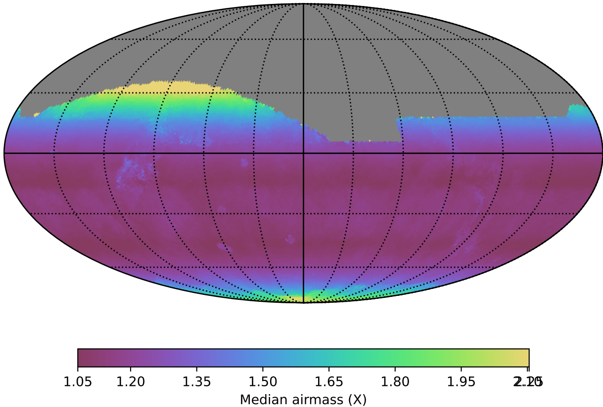
roll_pause_mjdp270_v3.4_10yrs All sky i band: Median airmass
