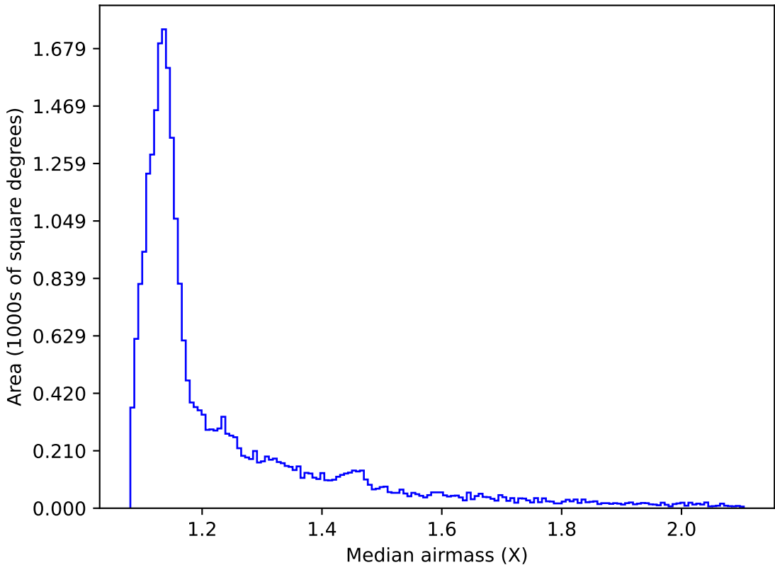
roll_pause_mjdp270_v3.4_10yrs All sky i band: Median airmass
