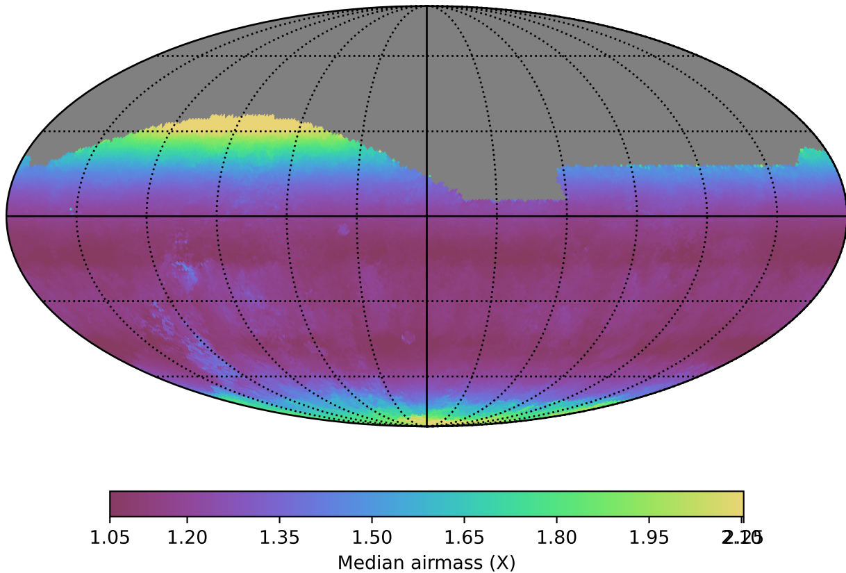
roll_pause_mjdp270_v3.4_10yrs All sky g band: Median airmass
