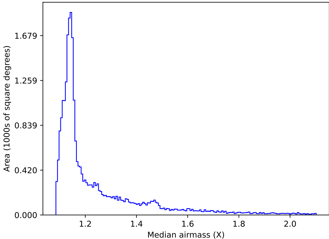
roll_pause_mjdp270_v3.4_10yrs All sky all bands: Median airmass
