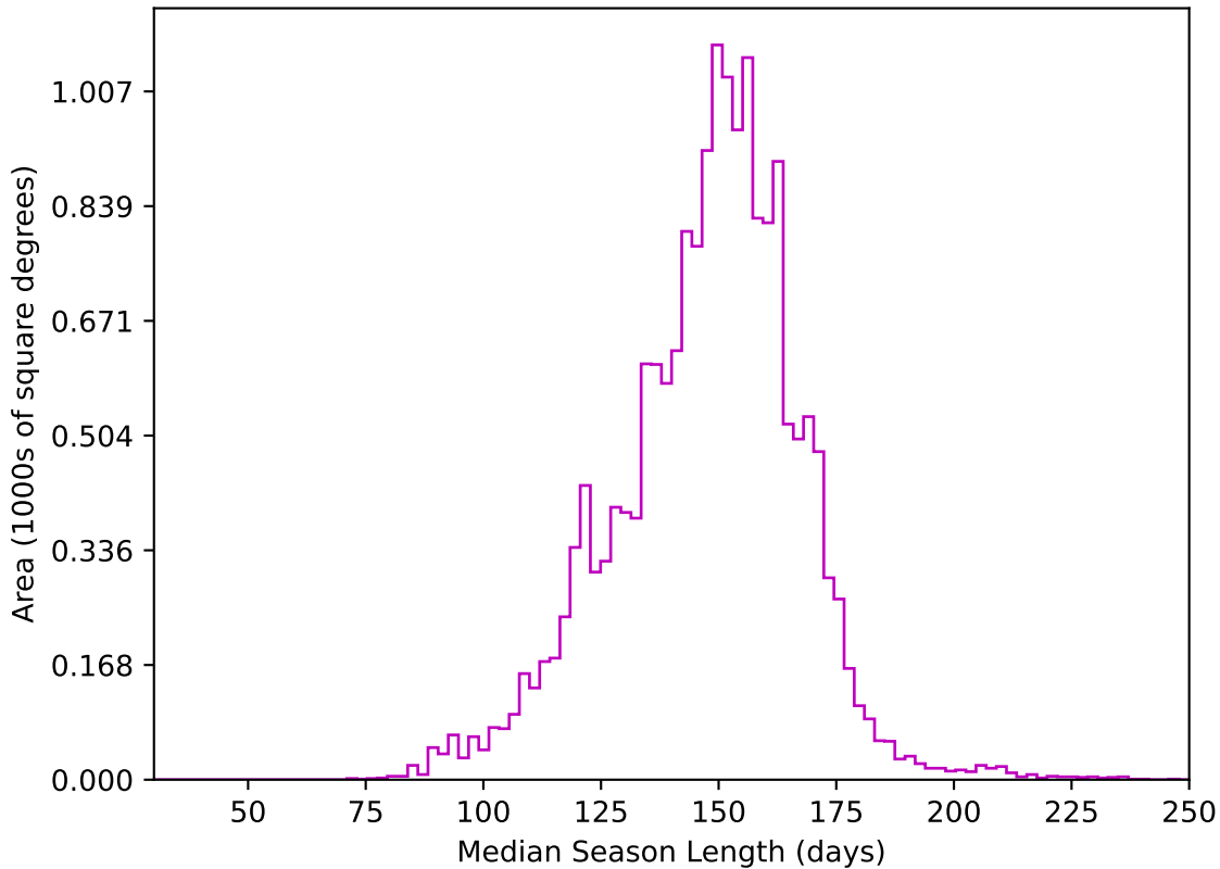
roll_pause_mjdp270_v3.4_10yrs WFD z band: Median Season Length
