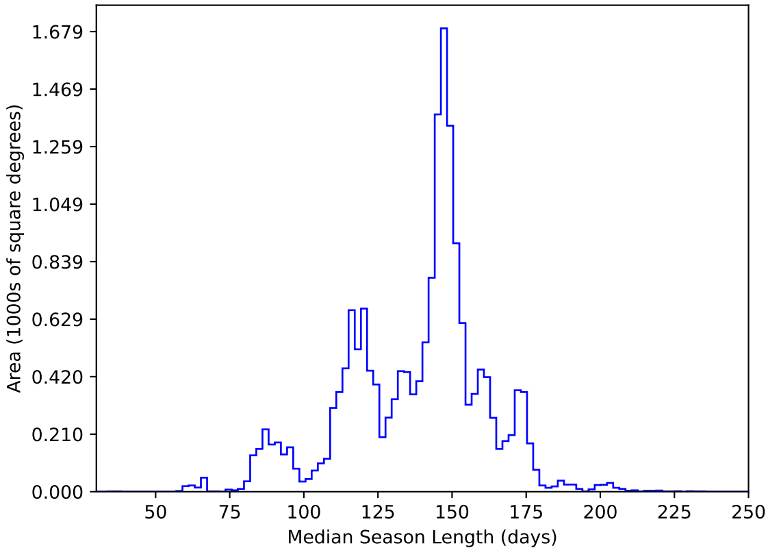
roll_pause_mjdp270_v3.4_10yrs WFD y band: Median Season Length
