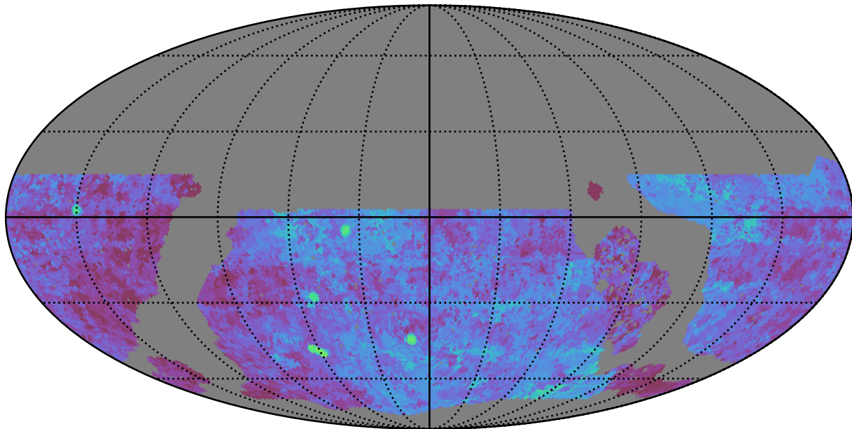
roll_pause_mjdp270_v3.4_10yrs WFD u band: Median Season Length
