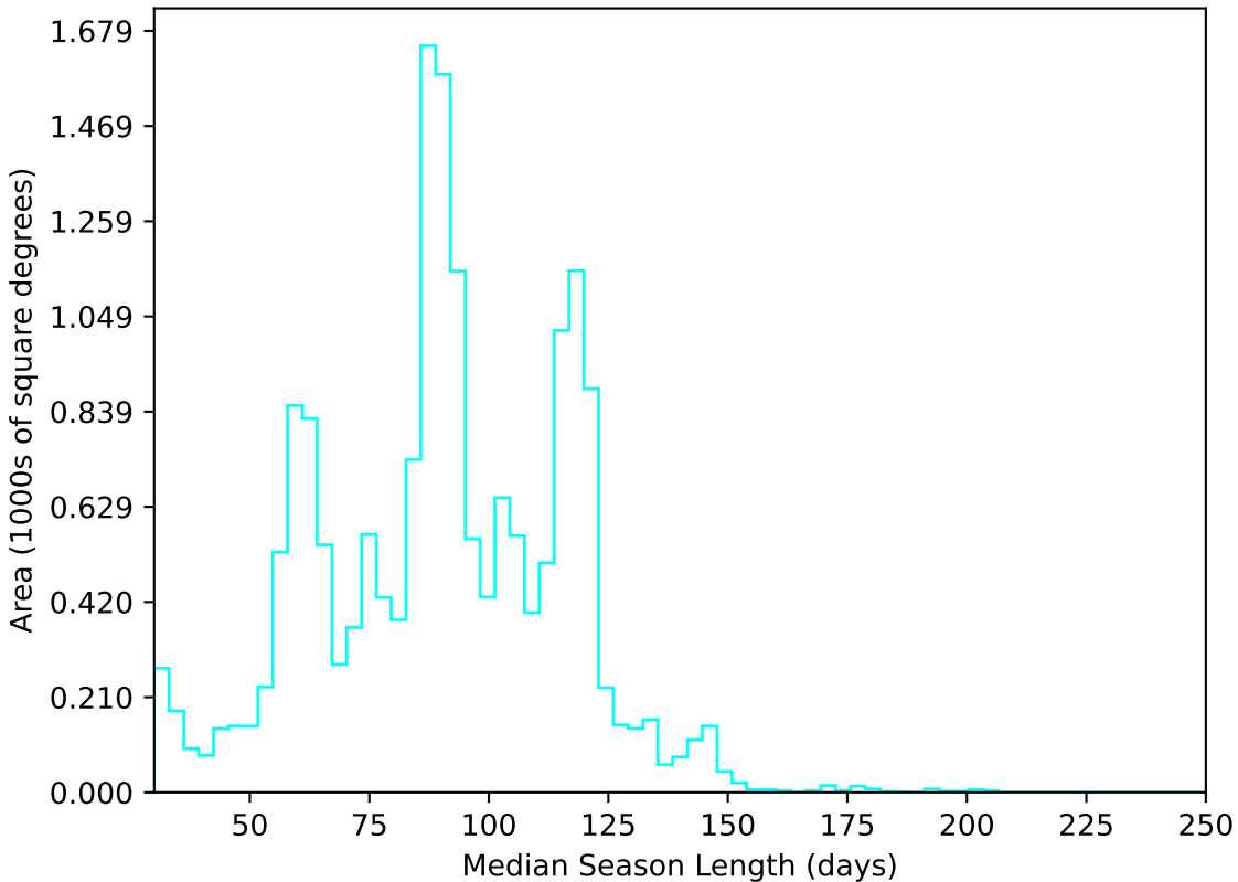
roll_pause_mjdp270_v3.4_10yrs WFD u band: Median Season Length
